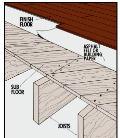
Fig. 4. Wood joist construction using square-edge board subfloor.
