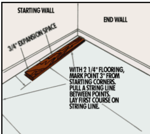
Fig. 5. Establishing starter line for nailing first strip.
