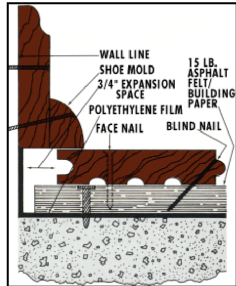
Fig. 1. Plywood-on-slab method of installing strip oak flooring
