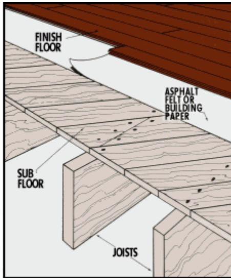
Fig. 4. Wood joist construction using square-edge board subfloor.
